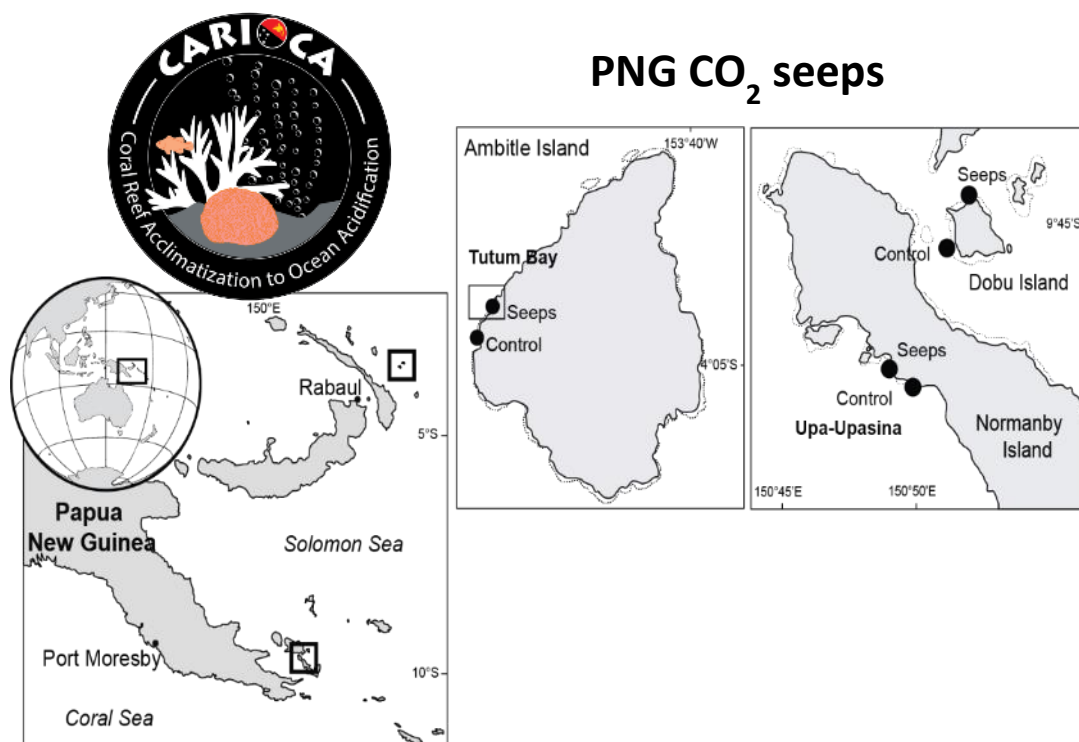
Fig. 4.8.1. Localisation of the two volcanic sites where the CARIOCA project studied the effect of CO 2 seep emissions on coral reefs.
