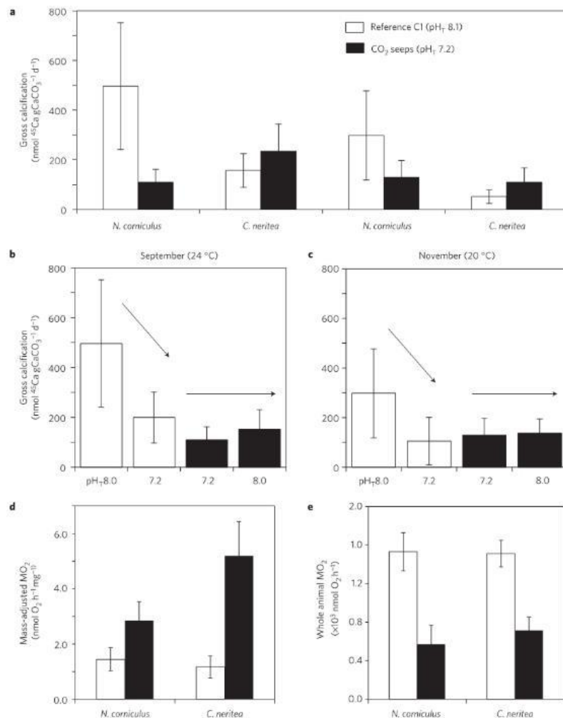
Fig. 4.7.2. Gross calcification (GC) and metabolic oxygen consumption (MO 2 ) in Nassarius corniculatus and Cyclope neritea across normal and acidified sites. A. GC in September and November at pH measured at collection sites. b-c. GC of N. corniculatus in September (a) and November (b) to measure the response of samples collected within the seeps and at Reference site and incubated at crossed pH treatments. Arrows show the GC change on samples incubated at pH of collection (CO 2 seeps or Reference C1 sites) and the pH of the incubation (pH T 8.0 and 7.2). Oxygen uptake as an index of MO 2 expressed as body mass adjusted MO 2 ( d ) and whole animal MO 2 ( e ).
