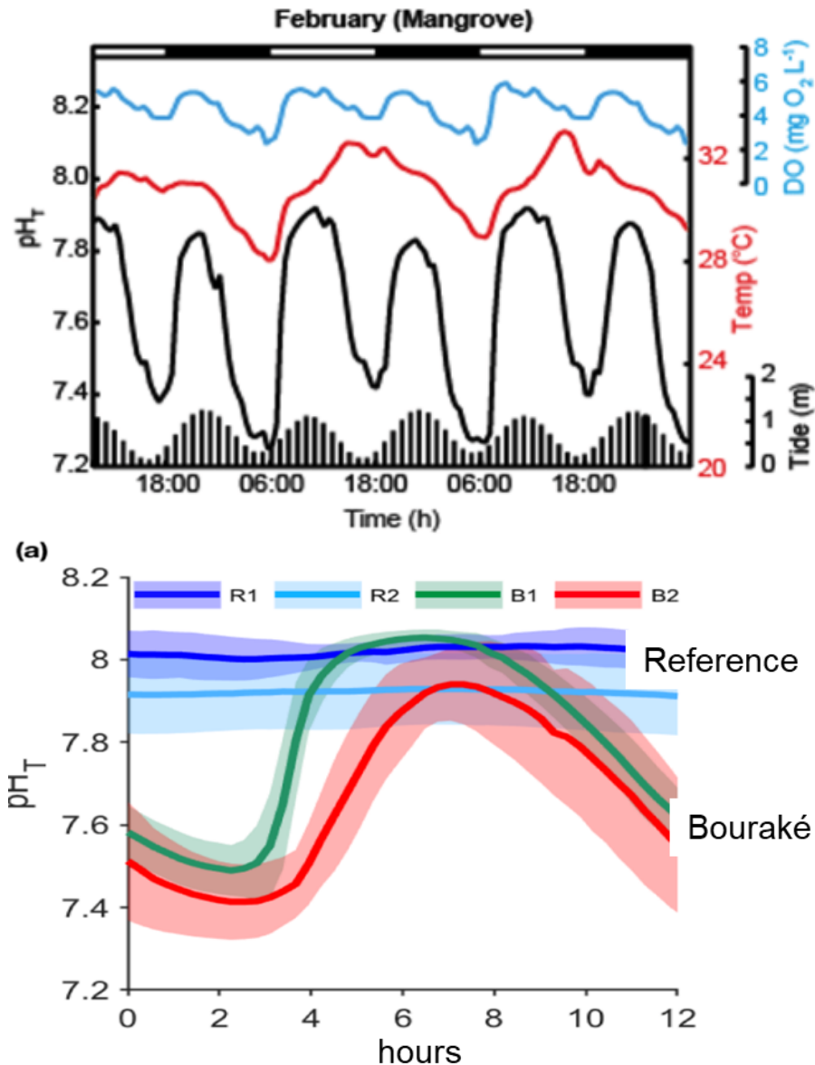
Fig. 4.10.3. The graph on the top shows the seawater \text{pH}_T , temperature, oxygen changes and tide measured in February 2017 during a 3-day cycle in Bouraké. On the bottom, seawater \text{pH}_T variations were recorded at the reference (Sts R1 and R2) and Bouraké (Sts B1 and B2) reefs. Data were overlaid at a single tidal phase (12 h). Data are 22, 72, 31, and 72 semidiurnal tidal cycles.
