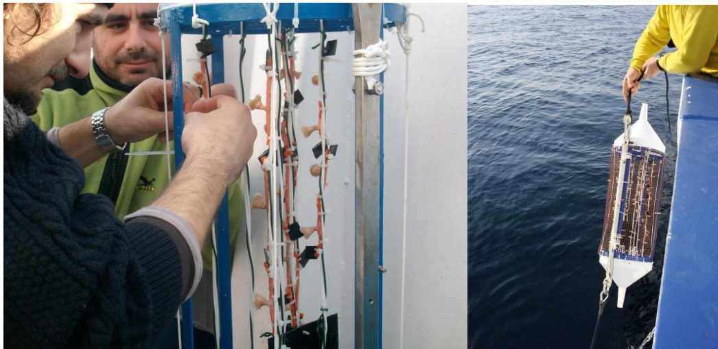
Fig. 4.6.1. Transplantations of D. dianthus suspended at 350 m depth on a mooring off Corsica.
