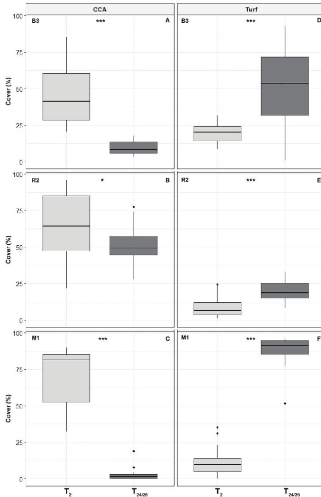
Fig. 4.11.1. Change in crustose coralline algae (CCA) (A, B, and C) and Turf percent cover (D, E, and F) on top sides of the tiles between the beginning (two months after the time of deployment, T 2 ) and the end (after ca two years of deployment, T 24/26 ) of collector deployment at study stations B3, R2 and M1 (number of tiles n = 15, 20 and 19, respectively). Data are median values ± 25th and 75th percentiles (box), minimum and maximum values (whiskers), and outliers (dots). Stars represent statistical significance.
