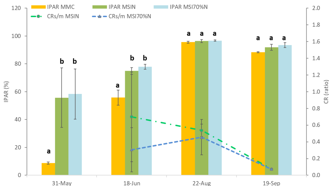
Figure 4.1 IPAR and CR s/m per treatment during the maize cycle. MMC: Maize monoculture, MSI: Maize-stylo intercropping, MSI 70%N : Maize-stylo intercropping with 70% N fertilisation. IPAR: Intercepted photosynthetically active radiation (%), CR s/m : Competitive ratio of stylo relative to maize. n=9 for each treatment. Different letters indicate significant difference according to ANOVA (P < 0.05).
