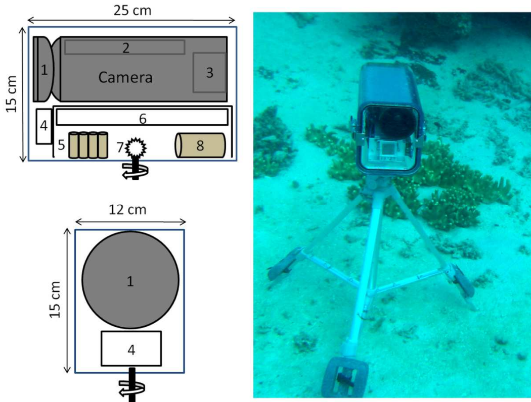
Figure 1. The MICADO system. On top left: side view of MICADO, bottom left: front view and on the right: picture of MICADO underwater. 1: Wide angle lens; 2: internal hard drive of the camera; battery of the camera; 4: Timer; 5: rechargeable batteries to power the electronic card and the timer, 6: control circuit commanding the entire system; 7: engine inducing the rotation; and 8: 1,5V battery powering the engine.
