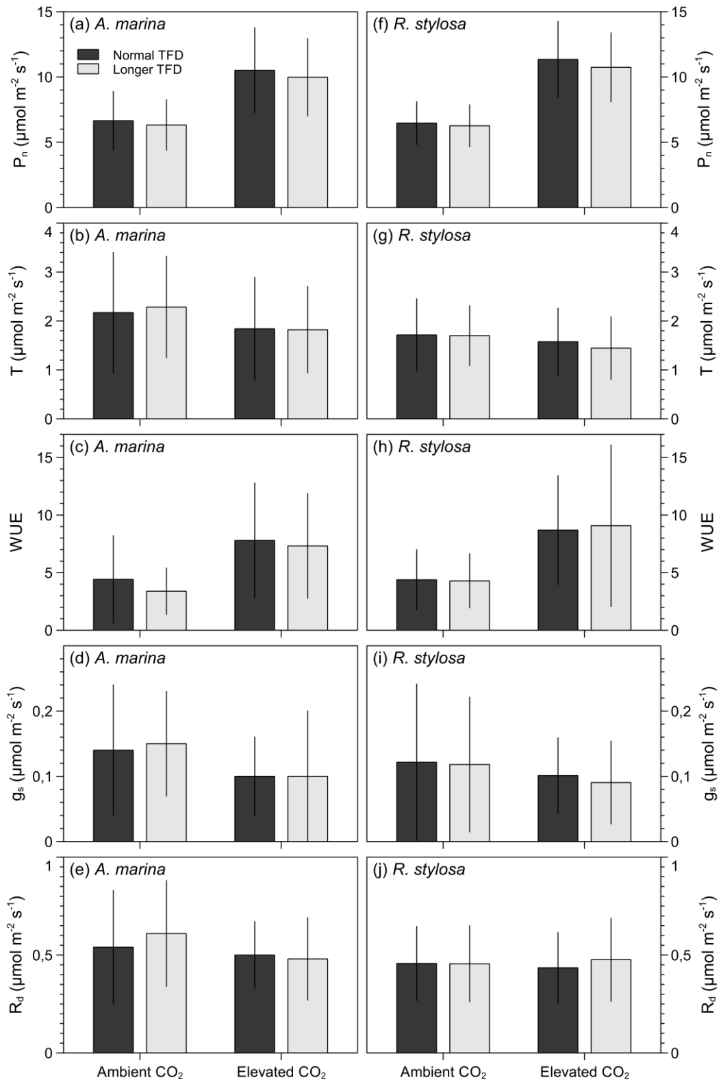
Fig. IV-3: Mean values ( \pm SD) of leaf gas exchange parameters for A. marina and R. stylosa grown in ambient (400 ppm) or elevated (800 ppm) CO 2 , and under normal (dark-grey bars) and longer TFD (grey bars), for 12 months. (a and f) photosynthetic rates ( \mu\text{mol m}^{-2} \text{s}^{-1} ), (b and g) transpiration rates ( \mu\text{mol m}^{-2} \text{s}^{-1} ), (c and h) water-use efficiency, (d and i) stomatal conductance ( \mu\text{mol m}^{-2} \text{s}^{-1} ), and (e and j) dark respiration rates ( \mu\text{mol m}^{-2} \text{s}^{-1} ).
