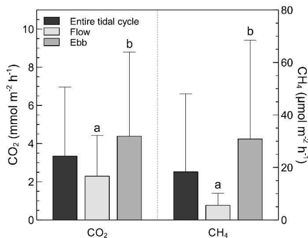
Fig. III-7: Mean CO 2 (mmolC m -2 h -1 ) and CH 4 (μmolC m -2 h -1 ) (+SD) emissions during the complete tidal cycles ( n=284 ), the flow tides ( n=141 ) and the ebb tides ( n=143 ) in the mangrove of Ouemo for the period December 2016 to September 2017. Different letters indicate significant differences (two-samples t-test, CO 2 : t_{(205,66)}=5.11 , p<.001 , CH 4 : t_{(146,3)}=7.96 , p<.001 ).
