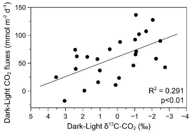
Fig. III-6: Difference in dark and light fluxes ( \text{mmol m}^{-2} \text{d}^{-1} ) as a function of the difference between dark and light \delta^{13}\text{C-CO}_2 (‰). n=25 , each point representing the mean of three replicates.
