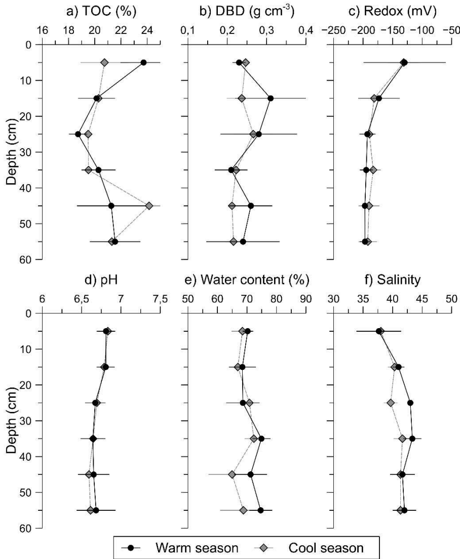
Fig. III-2: Physicochemical profiles measured in January (black lines) and in June (grey dotted lines) 2017. Each point is the mean of three replicates ± SD.
