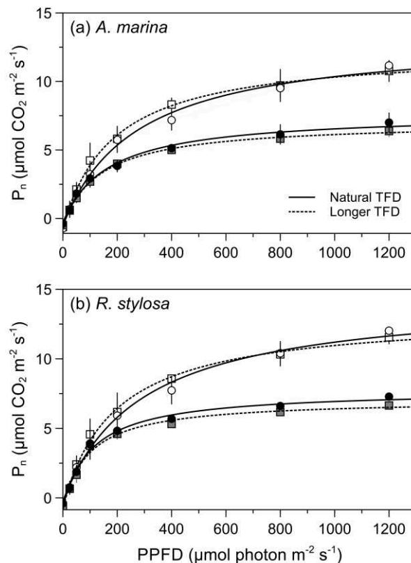
Fig. IV-6: P n /PPFD curves for A. marina (a) and R. stylosa (b) at the end of the experiment. ( n=3 \pm SD). Colored markers: ambient CO 2 concentrations, white markers: elevated CO 2 concentrations.
