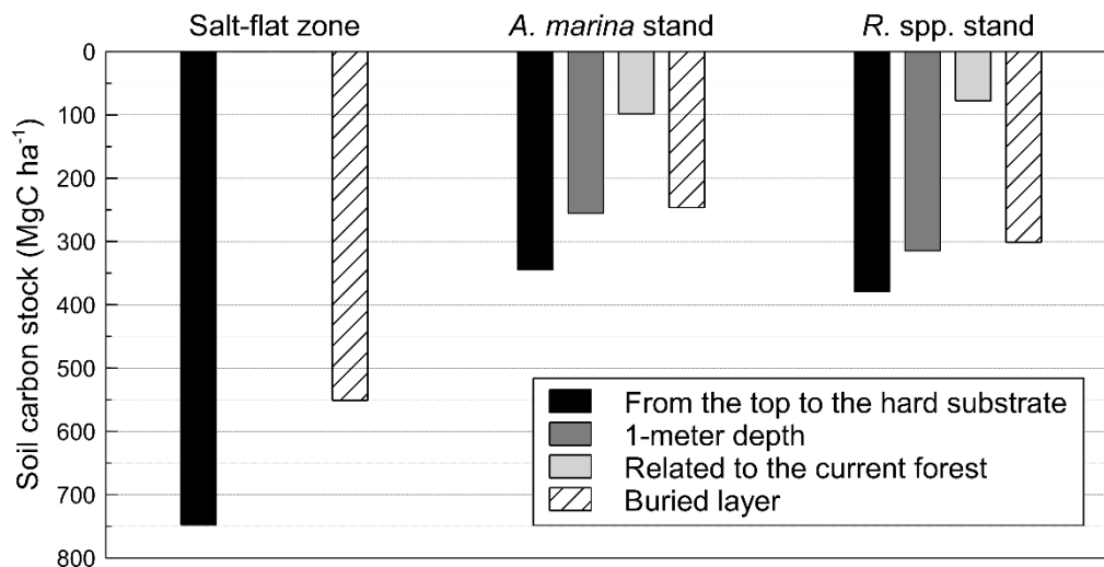
Fig. II-7: Figure 5: Representation of the soil carbon stocks (MgC ha -1 ) for different sediment layers at the three zones: salt-flat, A. marina stand, and R. spp. stand. Concerning the stocks related to the current forest, carbon stocks were integrated from 0 to 35 cm and from 0 to 25 cm under A. marina and R. spp. , respectively. Regarding the buried layer, carbon stocks were integrated from 70 cm to 265 cm in the salt-flat zone, from 35 to 140 cm in the A. marina stand, and from 25 to 125 cm in the R. spp. stand.
