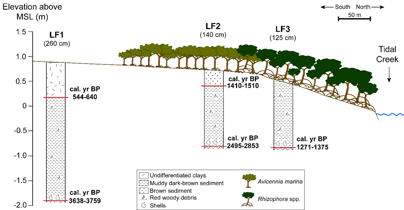
Fig. II-4: Stratigraphic profiles of cores LF1, LF2 and LF3, and mangroves species distribution along a South-North transect. MSL: Mean Sea Level.
