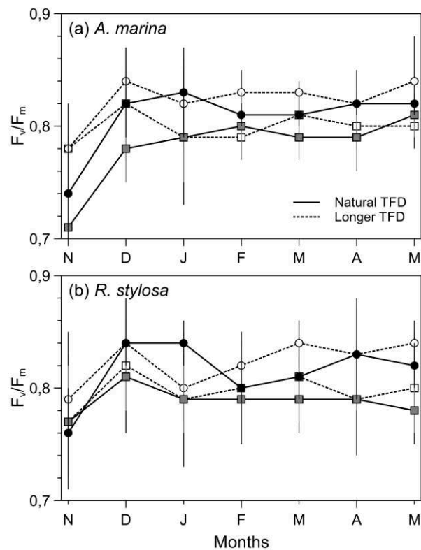
Fig. IV-7: Maximum quantum efficiency of PSII photochemistry ( F_v/F_m ) for A. marina (a) and R. stylosa (b) from November 2016 to May 2017. ( n=30 \pm SD ). Colored markers: ambient CO 2 concentrations, white markers: elevated CO 2 concentrations.
