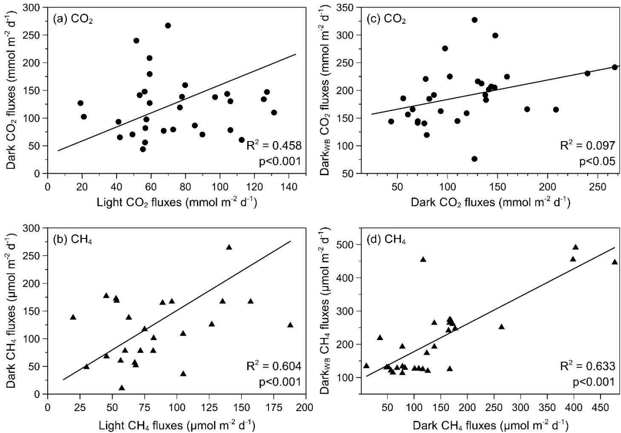
Fig. III-3 : (a) and (b): Relationship between light and dark fluxes of CO 2 (mmol m -2 d -1 ) and CH 4 (μmol m -2 d -1 ); (c) and (d): Relationship between dark fluxes without the upper 1-2 mm of soil (Dark WB ) and dark fluxes of CO 2 (mmol m -2 d -1 ) and CH 4 (μmol m -2 d -1 ); n=35, each point is the mean of three replicates.
