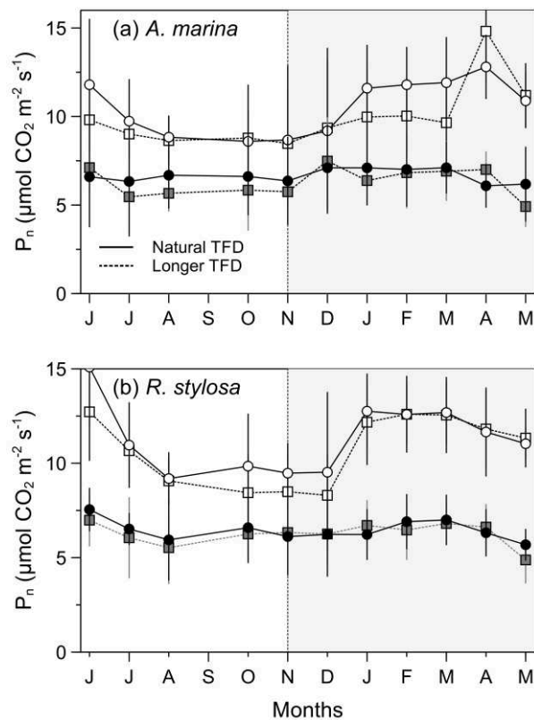
Fig. IV-4: Annual evolution ( \pm SD) of leaf net photosynthetic rates (P n , \mu\text{mol m}^{-2} \text{s}^{-1} ) for (a) A. marina , and (b) R. stylosa . Colored markers: ambient CO 2 concentrations, white markers: elevated CO 2 concentrations. Shaded area represents the warm season.
