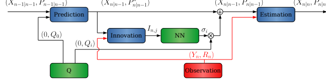
Fig. 2. Schematic representation of the proposed filter (NNAKF). Input data is represented in red, and trainable components of the filter are represented in green.
