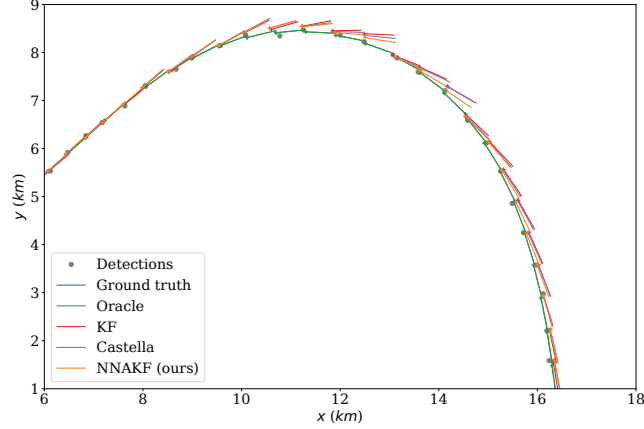
Fig. 3. Example of tracking results projected in the horizontal plane. For each filter, estimated position is represented by a cross and the estimated velocity by a speed vector. Oracle’s output and the ground truth are almost indistinguishable. It seems on this particular trajectory that the NNAKF adapts quicker to the turn while it is stable during straight lines.
