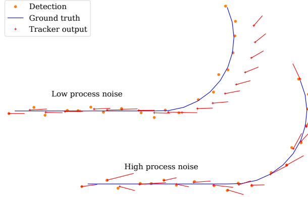
Fig. 1. Two-dimensional example of filtering using a Kalman filter with a Constant Speed model and two different settings of the noise process. Blue line is the real trajectory, orange dots are the detections provided to the filter, and red crosses and lines represent (respectively) the estimated states and the estimated velocity vectors.
