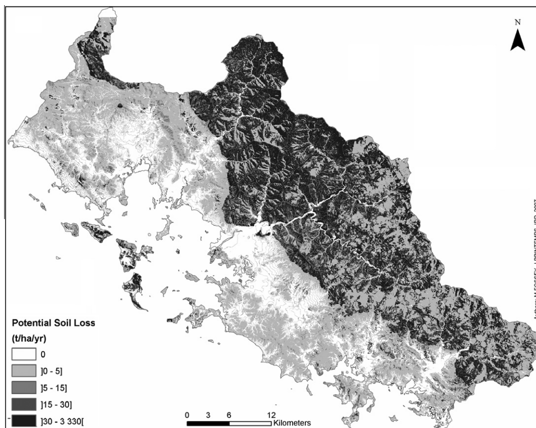
Fig. 6. Spatial distribution map of average annual potential soil loss with the Universal Soil Loss Equation. The average of soil losses is 18 t/ha/yr. At the difference of multi-criteria analysis, the dichotomy between the coastal plain and the ultramafic massifs is more characterised on this map.
